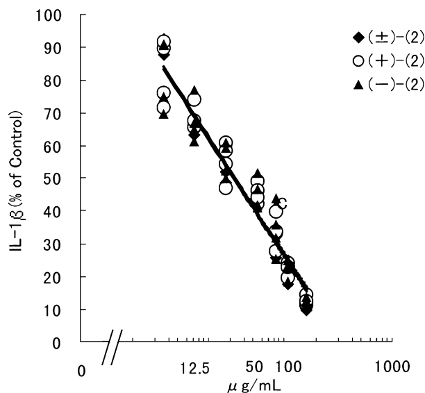
Figure 4. Suppressive effect of optical isomers of 2 1,1-dimethyl-3-oxobutylammonium salt on IL-1β production in THP-1 cells. IC 50 (95% C.I.). (±)-2 1,1-dimethyl-3-oxobutylammonium salt: 29.6 (26.6–32.9) μg/mL; (+)-2 1,1-dimethyl-3-oxobutylammonium salt: 30.8 (27.9–33.9) μg/mL; (-)-2 1,1-dimethyl-3-oxobutylammonium salt: 30.4 (26.8–34.3) μg/mL. Each symbol represents the production of IL-1β by THP-1 cells with various concentrations of optical isomers of 2 ( n = 4). Results were divided by the mean of the control. The mean and SE of the control were 109.4 ± 4.4 pg/mL. IC 50 and 95% confidence interval (CI) were determined by linear regression analysis.
