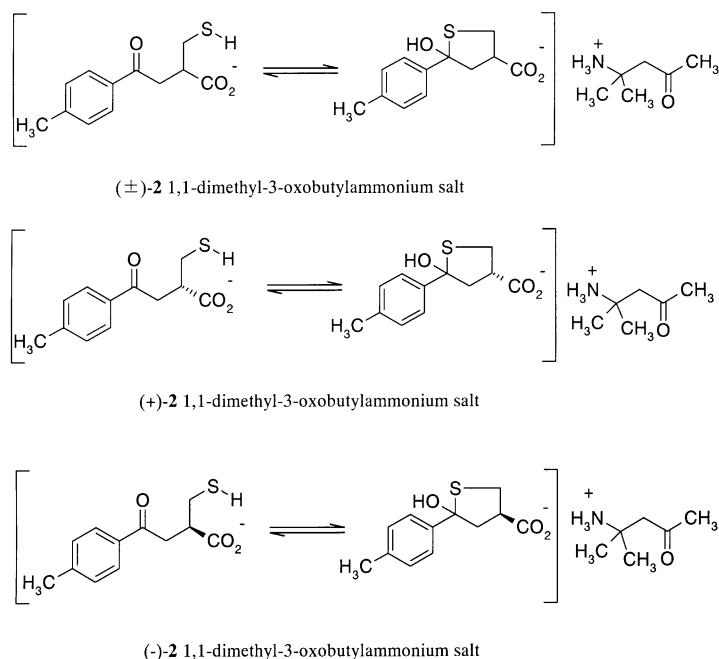
Figure 3. The structures of (±), (+), and (–)- 2 1,1-dimethyl-3-oxobutylammonium salt.
