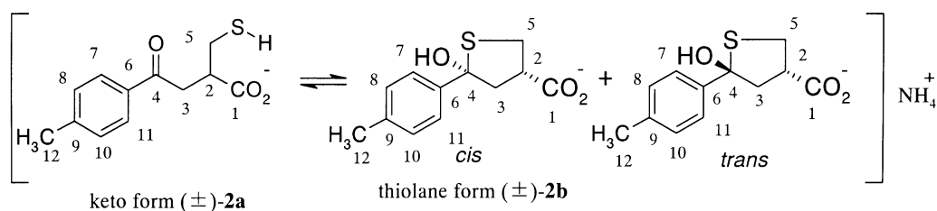
Figure 2. Keto form (±)- 2a and thiolane form (±)- 2b .
