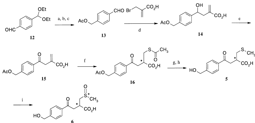
Scheme 5. Synthesis of metabolites 5 and 6 ; (a) NaBH 4 , EtOH, rt, 60 min; (b) Ac 2 O, pyridine, rt over:night; (c) H 2 SO 4 , THF–H 2 O, rt, 30 in, 96%; (d) indium metal, THF, 18–39 °C, 35 min, 87%; (e) CrO 3 , H 2 SO 4 , acetone–H 2 O, ice cooling, 10 min, 83%; (f) AcSH, Et 3 N, toluene, 60 °C, 2 h, 92%; (g) NH 3 , H 2 O, rt, 60 min; (h) CH 3 I, TOMAC, Et 2 O, rt, 30 min, 80%; (i) mCPBA, THF, ice cooling, 60 min, 77%.
