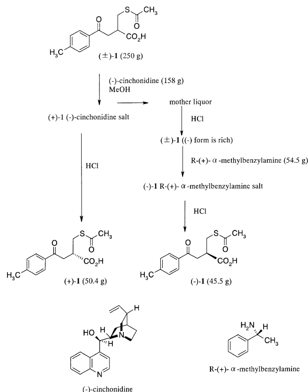
Scheme 3. Preparation of optically active esonarimod (1).
