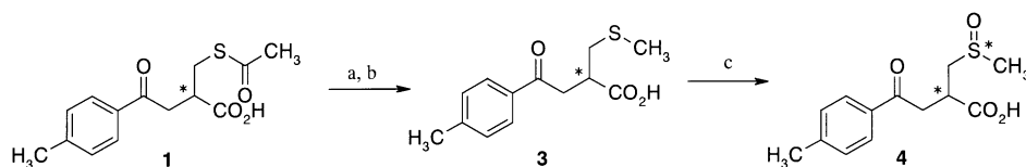
Scheme 4. Synthesis of metabolites 3 and 4 : (a) KOH, H 2 O, rt, 30 min; (b) CH 3 I, TOMAC, rt, 30 min, 80%; (c) mCPBA, THF, rt, 60 min, 37%.
