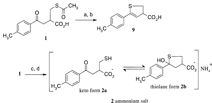
Scheme 2. Synthesis of 2 ammonium salt: (a) KOH or aqueous \text{NH}_3 (b) usual workup (acidification and extraction with organic solvent); (c) aqueous \text{NH}_3 -MeOH, 0-3\text{ }^\circ\text{C} , 5 min; (d) solvent removed under reduced pressure, 65%.
