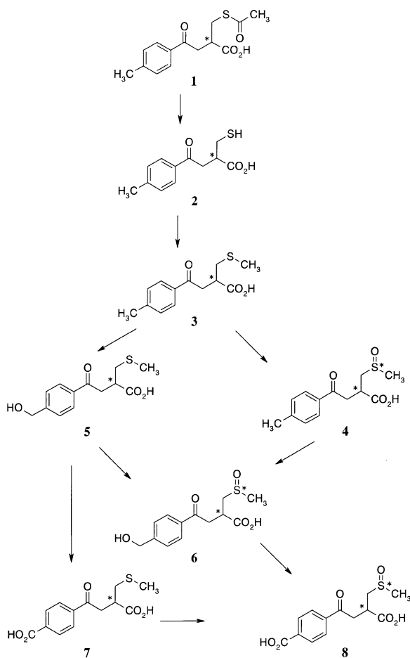
Scheme 1. A possible metabolic pathway of esonarimod ( 1 ) in rat.
