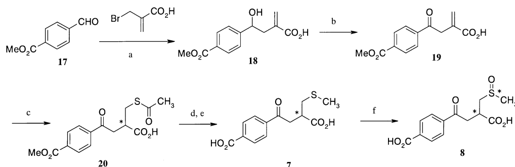
Scheme 6. Synthesis of metabolites 7 and 8 : (a) indium metal, THF, rt, overnight, 62%; (b) (COCl) 2 , DMSO, THF, Et 3 N, –74 °C, 10 min, 42%; (c) AcSH, Et 3 N, toluene, 60 °C, 40 min, 86%; (d) NH 3 , H 2 O, rt, 60 min; (e) CH 3 I, TOMAC, rt, 20 min, 61%; (f) mCPBA, THF, ice cooling, 40 min, 80%.
